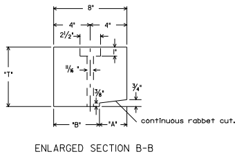
ENLARGED SECTION B-B
