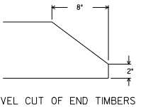
BEVEL CUT OF END TIMBERS
